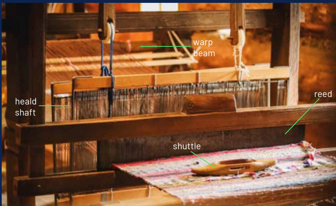
Above: A traditional loom with the warp beam, heald shafts, reed, and shuttle labeled. Photo by Zuzana Kacerová published August, 2019 and was retrieved from Unsplash in June of 2021.
